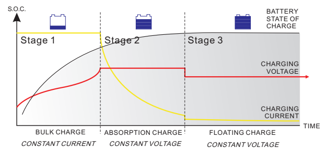
3-STAGE CHARGING DIAGRAM
